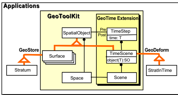
Fig. 7.23. Temporal extensions for GeoToolKit
